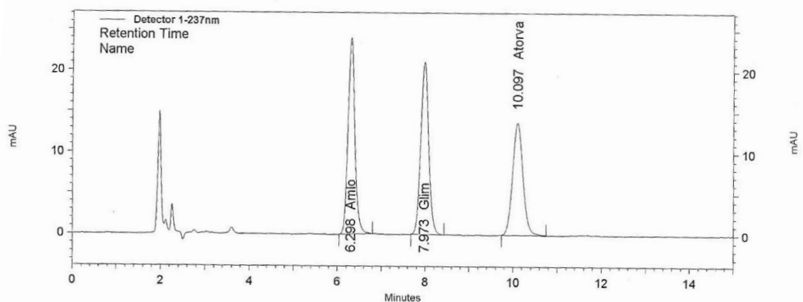
Figure 3.24. Chromatogram of amlodipine, glimepiride, and atorvastatin when setting the temperature at 22°C
